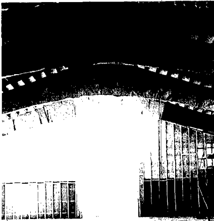
INTERIOR SKELETON of the sanctuary reveals the overhead beamwork. Made of bent wood, the exposed arches will enhance the interior finish.
